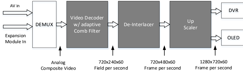
FIG 4. Signal Processing Path for Analog Input
